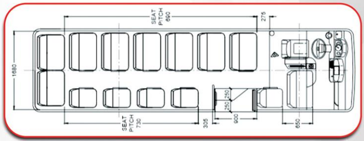
SEAT LAYOUT
